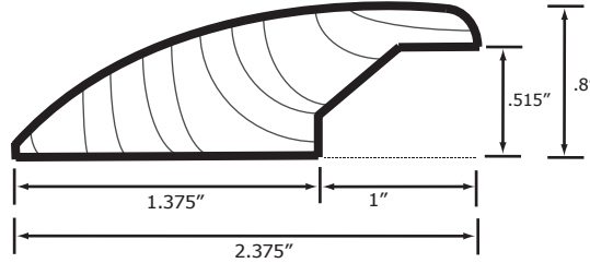
Lipover Reducer
