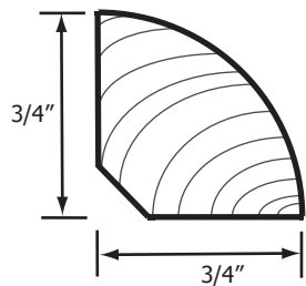
Quarter Round
