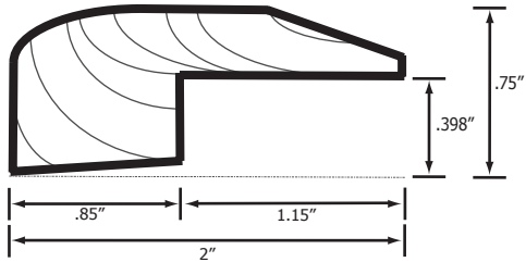
Baby Threshold/Carpet Reducer
